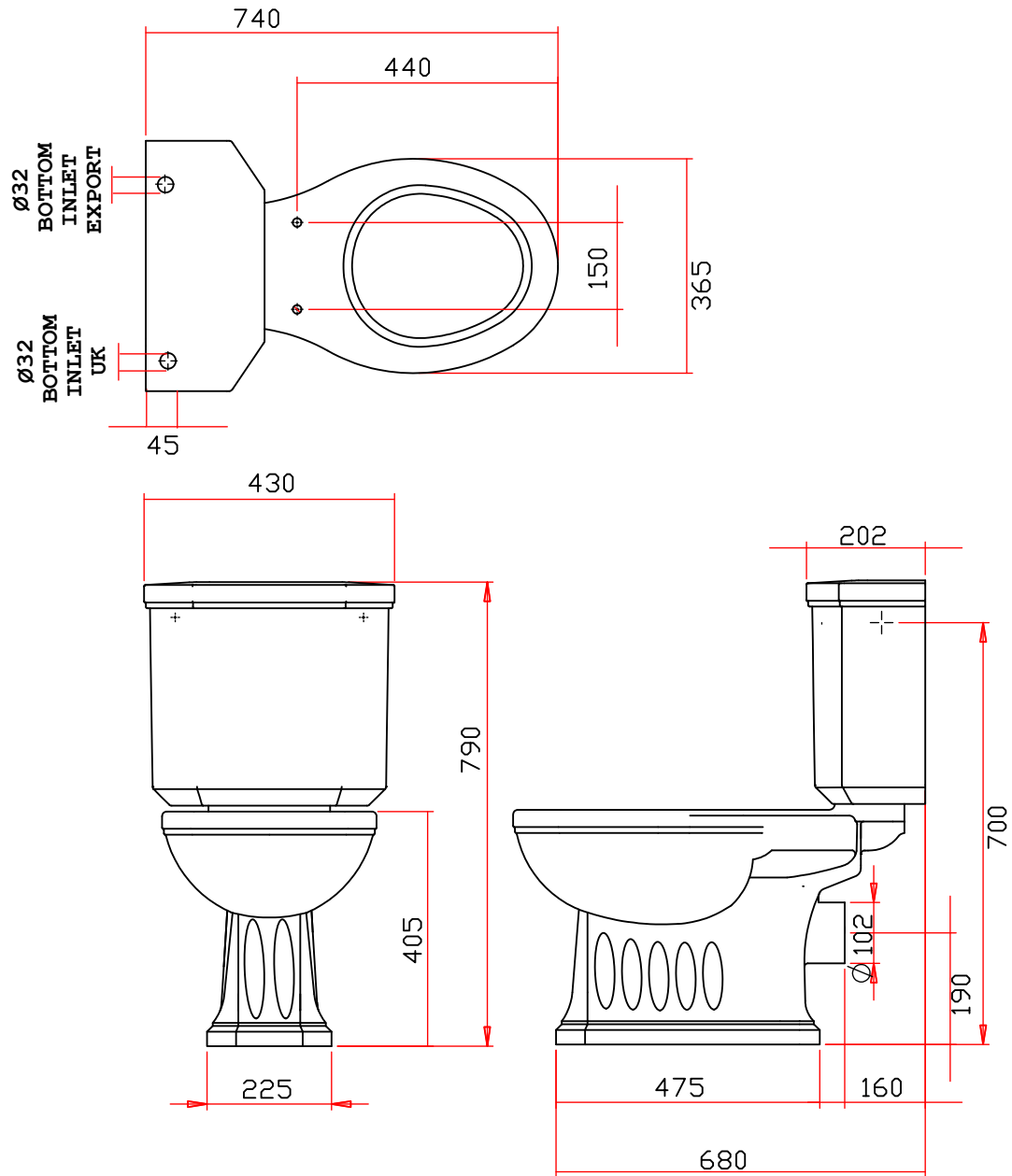
BELGRAVIA CLOSE COUPLED CLOSET AND CISTERN
