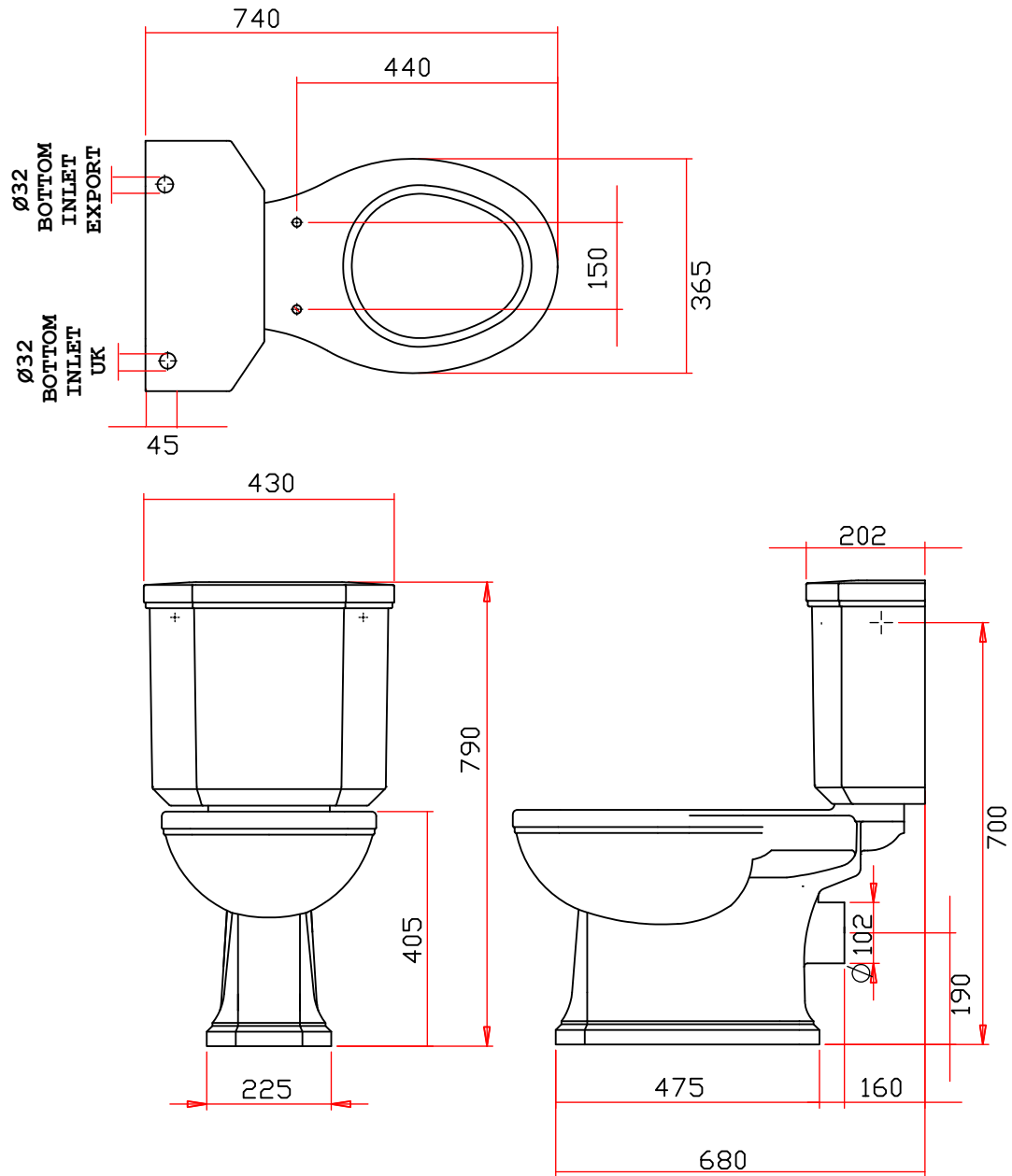
VICTORIAN CLOSE COUPLED CLOSET AND CISTERN
